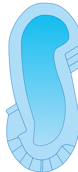
Hamal
